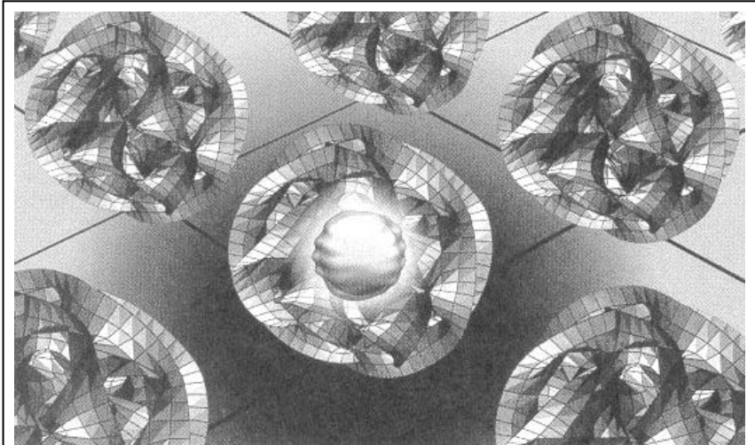
Figure 13.4 When a brane wraps around a sphere that is within the curled-up dimensions, it appears as a black hole in the familiar extended
